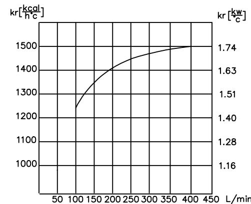
PERFORMANCE DIAGRAM
